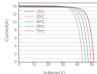
Current-Voltage Curve JAM72D30-555/GB
