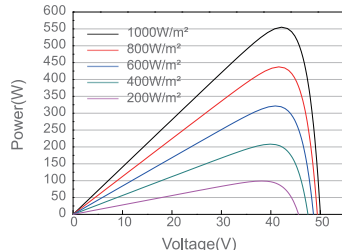
Power-Voltage Curve JAM72D30-555/GB
