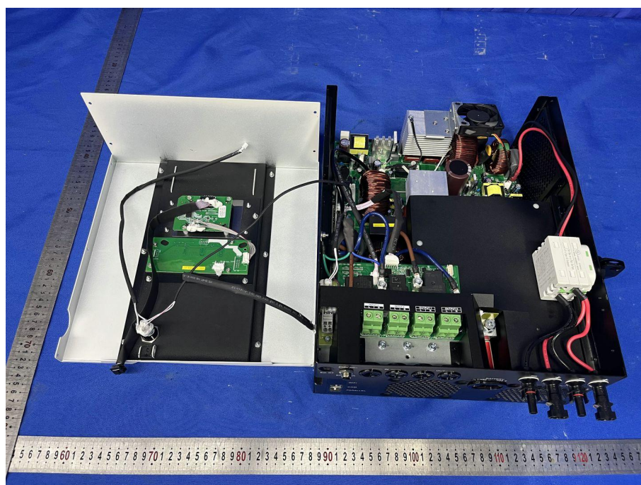
Fig. 6---Internal View
