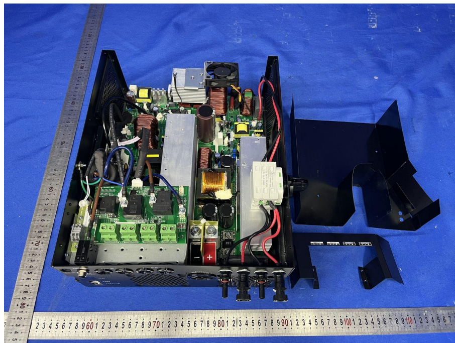
Fig. 7---Internal View
