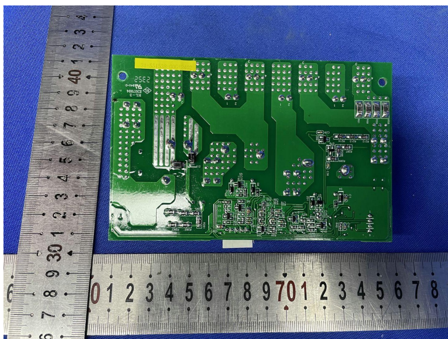
Fig. 10---PCB View
