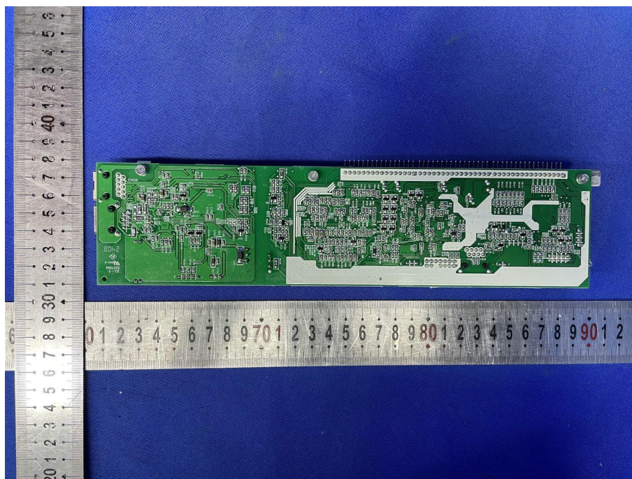
Fig. 20---PCB View
