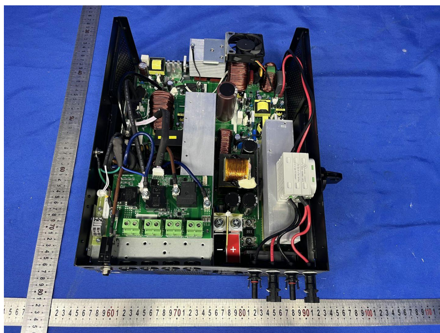
Fig. 8---Internal View
