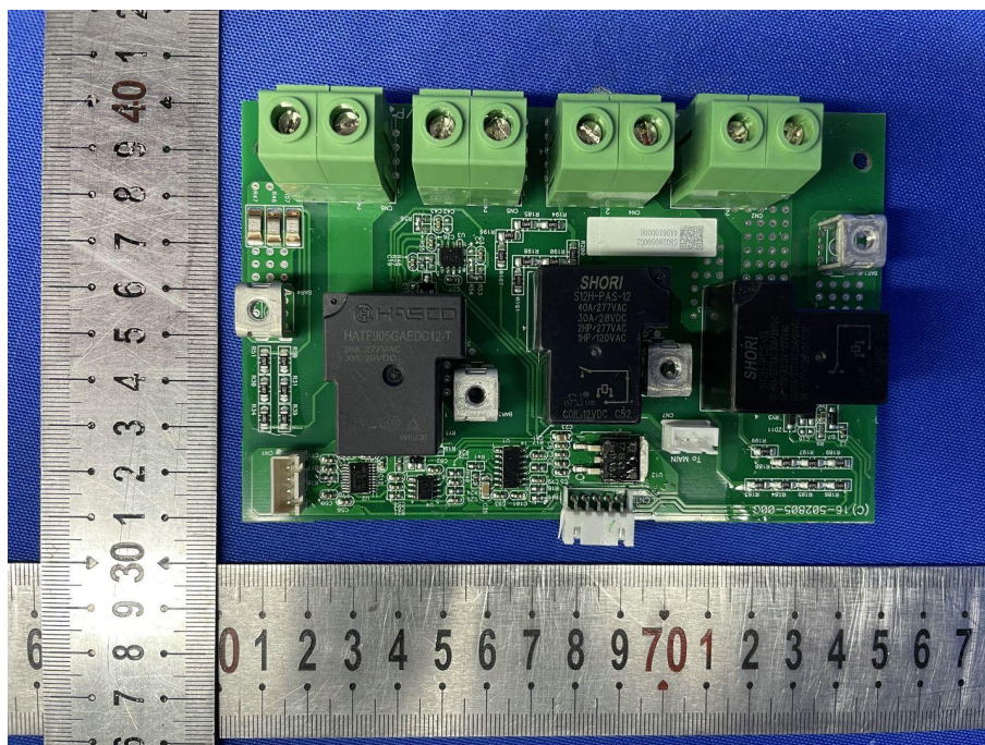
Fig. 9---PCB View
