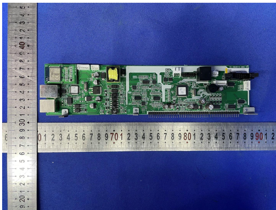
Fig. 19---PCB View
