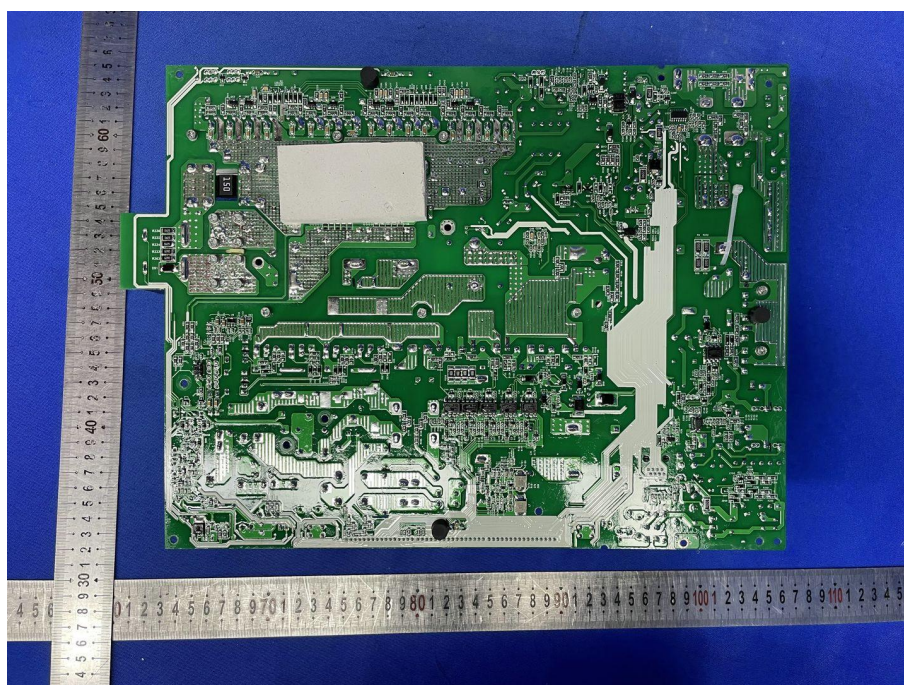
Fig. 18---PCB View
