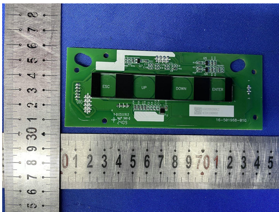
Fig. 13---PCB View
