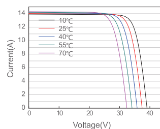
Current-Voltage Curve JAM54S30-415/GR
