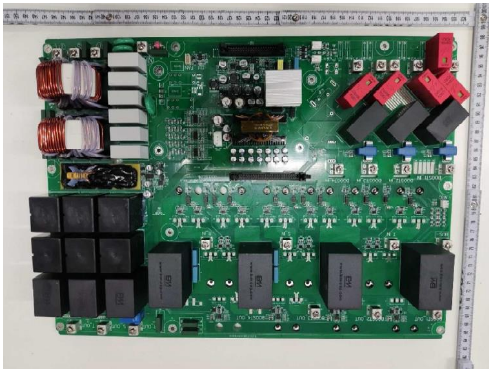
Front view of Main power board for R6-25K-T3-32, R6-30K-T3-32, R6-33K-T3-32, R6-36K-T3-32 (DC side with Surge Protector version)
