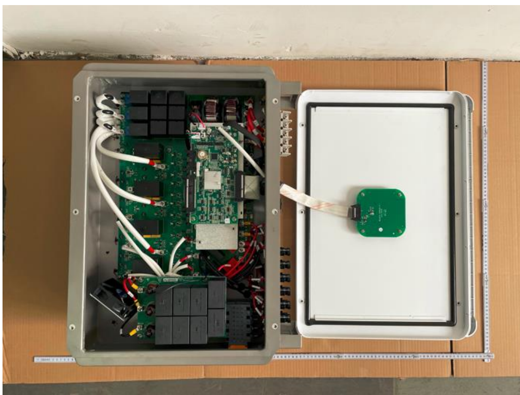
Internal view of R6-36K-T3-32, R6-33K-T3-32, R6-30K-T3-32, R6-25K-T3-32
