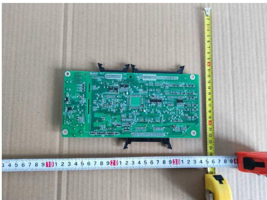
Back view of Control communication board
