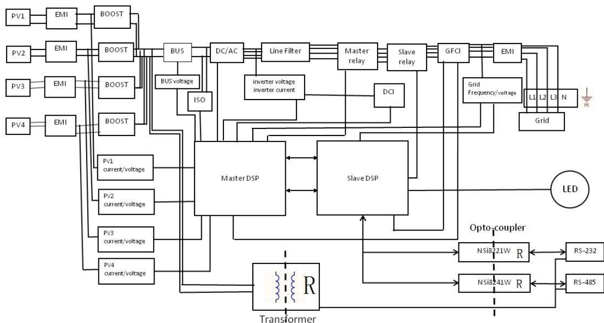
Figure 1 – Block diagram of the power circuit
