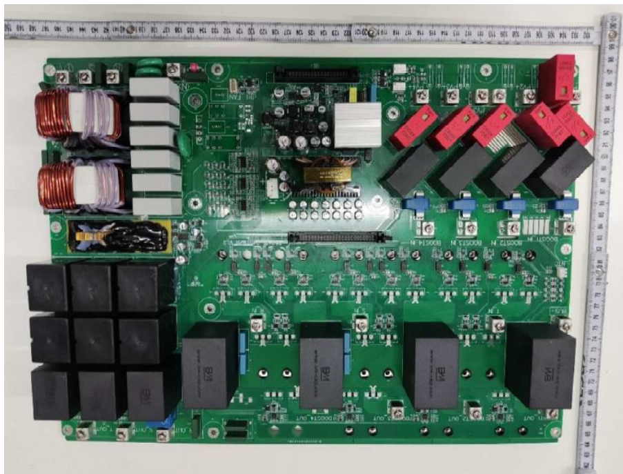
Front view of Main power board for R6-36K-T4-32, R6-40K-T4-32, R6-50K-T4-32 (DC side with Surge Protector version)
