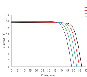
I-V Curve at Different Temperature SS8-72HD-590N
