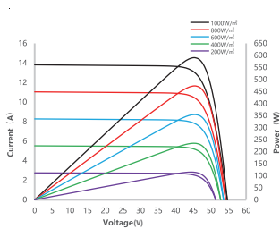
I-V/P-V Curve at Different Irradiation SS8-72HD-590N
