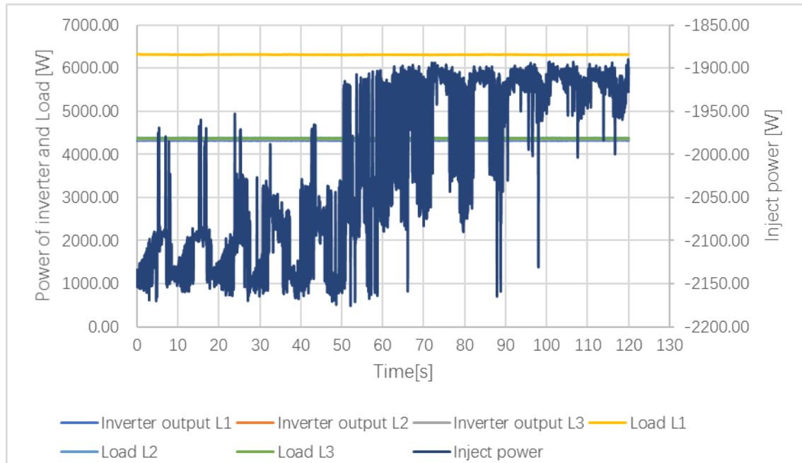
Graph_ (95%, 65%, 65%) load
