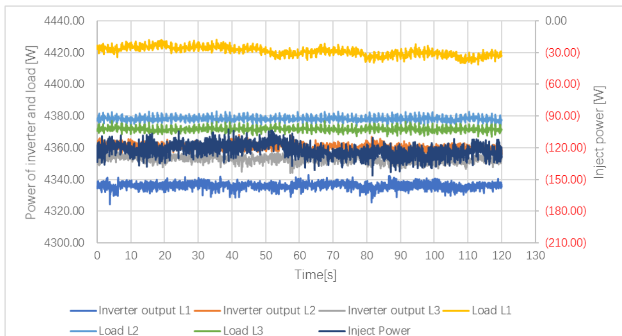
Graph_ (65%, 65%, 65%) load
