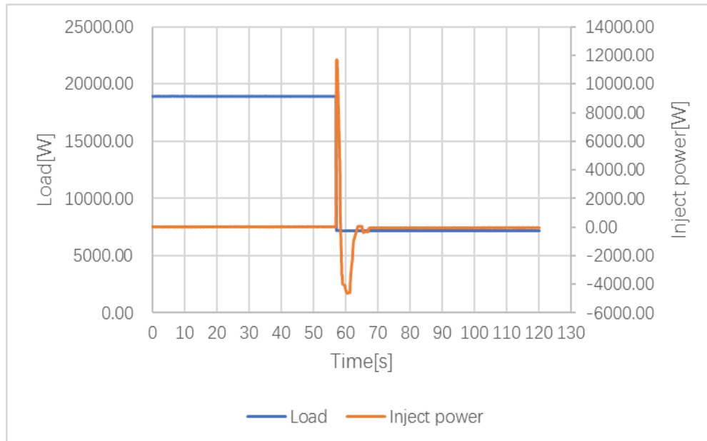
Graph 2_95% to 35%
