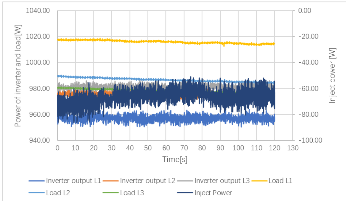
Graph_ (15%, 15%, 15%) load
