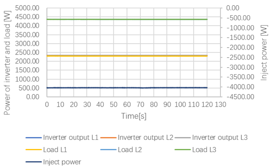
Graph_ (35%, 65%, 65%) load
