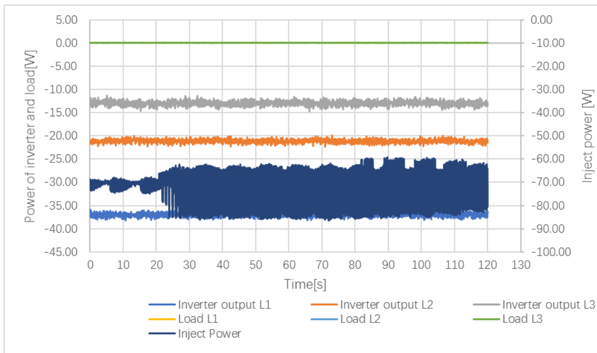
Graph_ (0%, 0%, 0%) load
